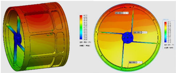
(a) 温度分布 (a) Temperature distribution
